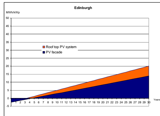
Figure 96 : Cumulative net energy production over system lifetime for Edinburgh
